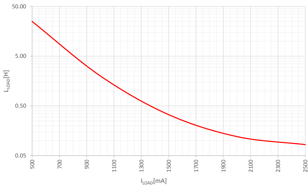
Figure 14. Typical single pulse demagnetization: L_{LOAD} vs I_{OUT} ( V_{CC} = 24\text{ V} , T_{AMB} = 125\text{ °C} )
