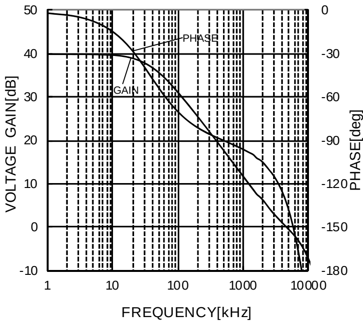
Figure 22. Voltage Gain - Phase - Frequency (VCC=7.5V/-7.5V, Av=40dB, RL=2k \Omega , CL=100pF, Ta=25°C)
