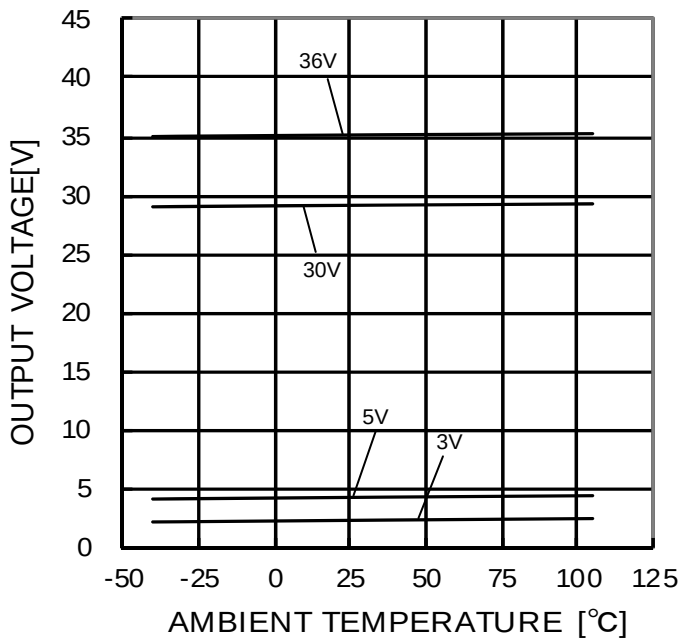
Figure 6. High level Output Voltage - Ambient Temperature ( R_L=10k\Omega )
