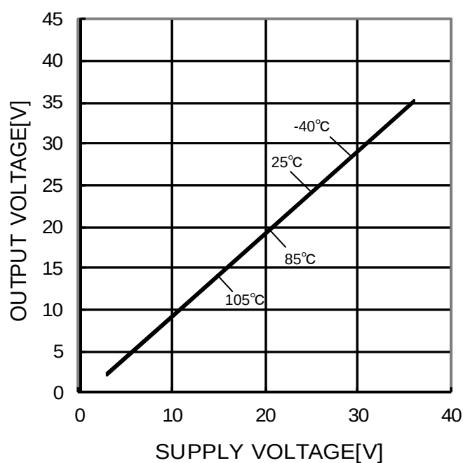
Figure 28. High level Output Voltage - Supply Voltage ( R_L=10k\Omega )
