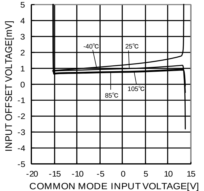
Figure 34. Input Common-mode Voltage Range (VCC/VEE=15V/-15V)
