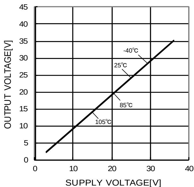
Figure 5. High level Output Voltage - Supply Voltage ( R_L=10k\Omega )
