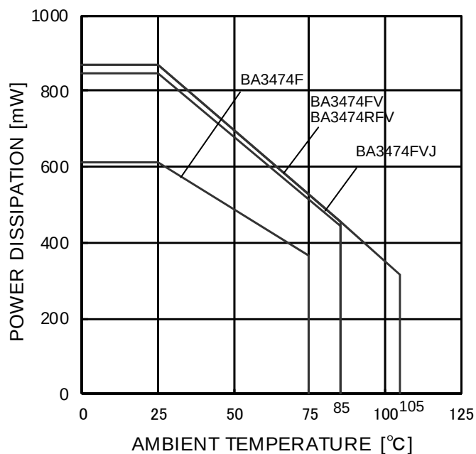
Figure 25. Derating Curve
