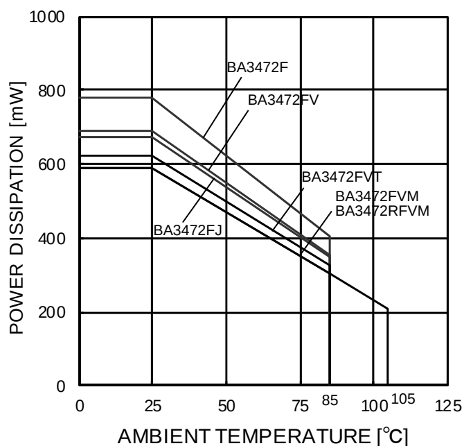
Figure 2. Derating Curve
