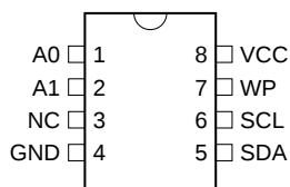
8-Pin PDIP
