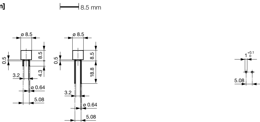
Drilling diagram
