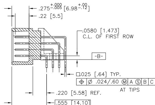
SECTION X-X
