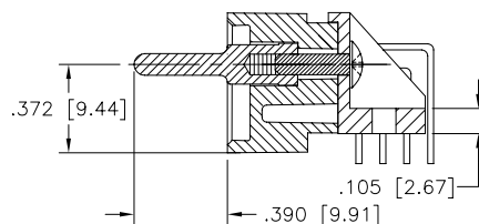
SECTION W-W
