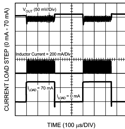
Load Transient I_{LOAD} = 0\text{ mA} to 70\text{ mA}
