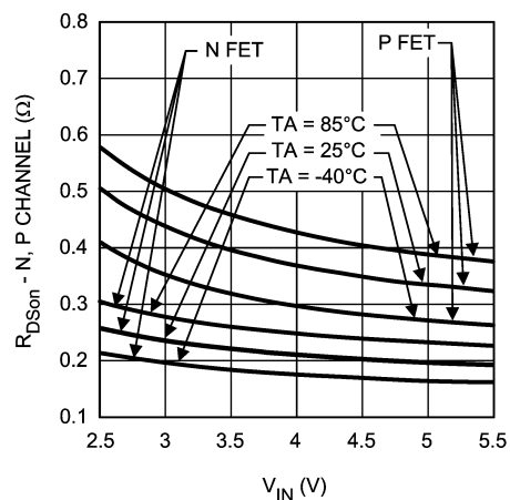
R_{DS(on)} vs. V_{IN} P & N Channel
