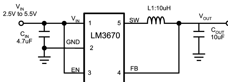
FIGURE 1. Fixed Output Voltage - Typical Application Circuit
