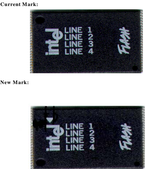
Figure 6. Mark for Pin-1 Indicator on 48-Lead 8-Mb, 16-Mb and 32-Mb TSOP
