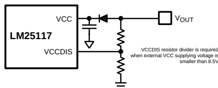
Figure 16. External VCC Supply For 5 V < V_{OUT} < 14.5 V
