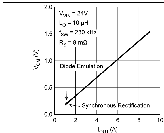
Figure 13. V_{CM} vs I_{OUT}
