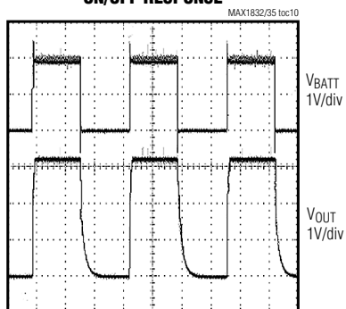
ON/OFF RESPONSE
