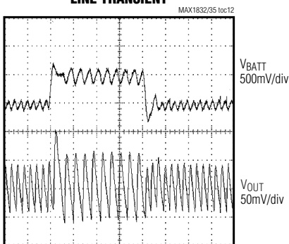
LINE TRANSIENT
