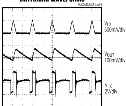
SWITCHING WAVEFORMS
