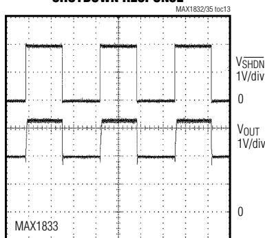
SHUTDOWN RESPONSE
