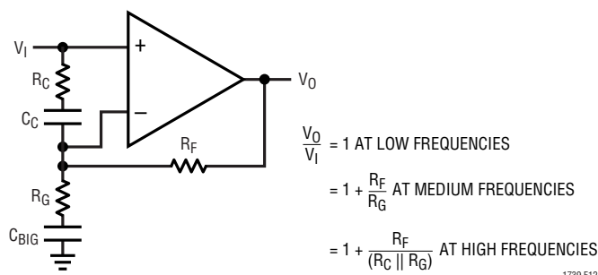
Figure 12. Combination Compensation
