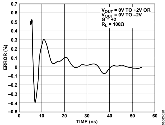
Figure 18. Settling Time
