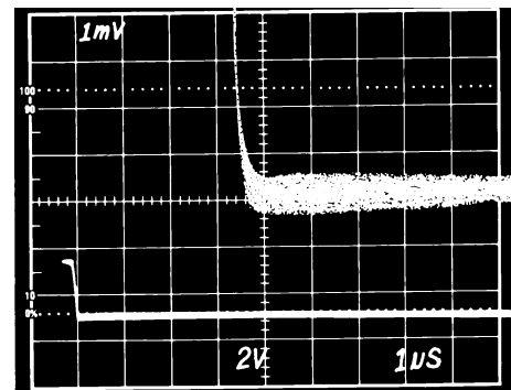
Negative-Going Settling Time ( V_{DD} = +15V , V_{SS} = -15V )
