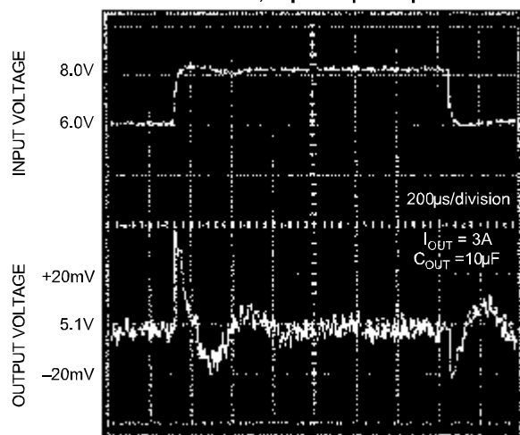
Line Transient Response with 3A Load, 10\mu F Output Capacitance
