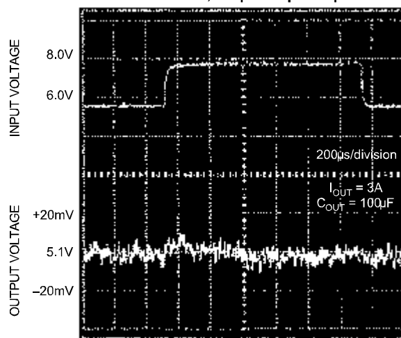
Line Transient Response with 3A Load, 100\mu F Output Capacitance
