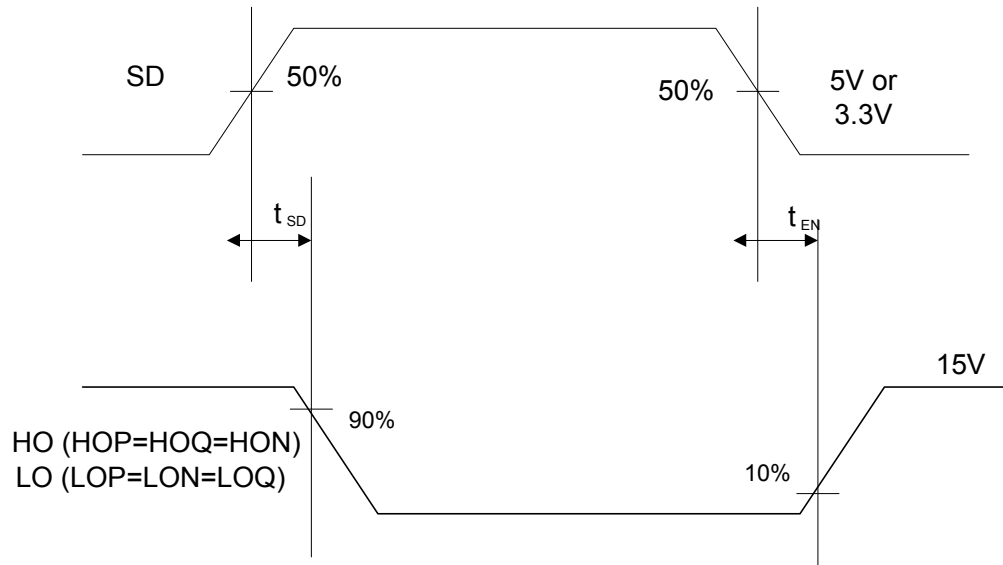
Figure 10 Shutdown Timing
