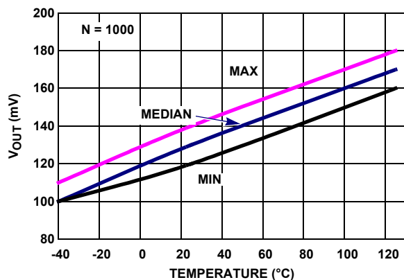
FIGURE 31. EL8171 V_{OUT} LOW vs TEMPERATURE, R_L = 1k , V_+ = 5V , V_- = 0V
