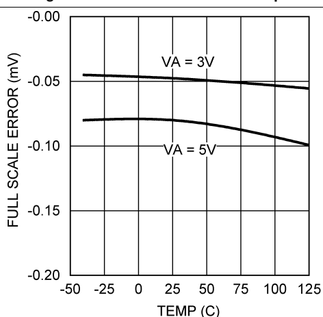
Figure 13. Full Scale Error vs Temperature
