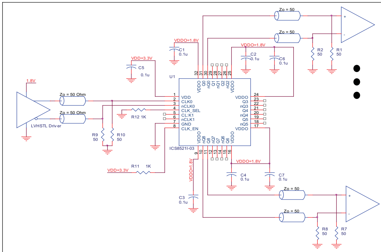
FIGURE 3A. 8521-03 SCHEMATIC EXAMPLE
