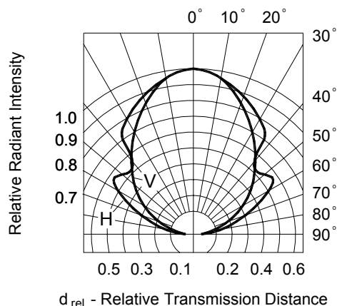
FIG.12 Directivity
