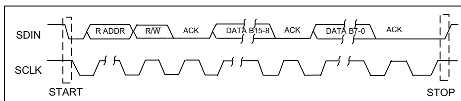
Figure 23 2-Wire Serial Interface
