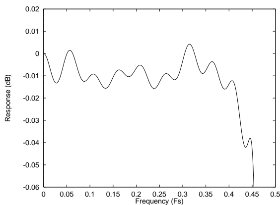
Figure 29 ADC Digital Filter Ripple –Type 1
