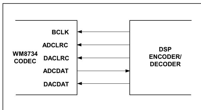
Figure 21 Slave Mode
