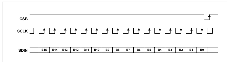
Figure 22 3-Wire Serial Interface
