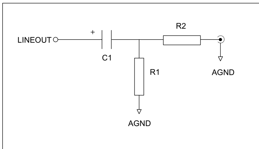
Figure 15 Line Outputs Application Drawing
