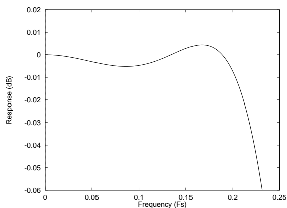
Figure 31 ADC Digital Filter Ripple –Type 2
