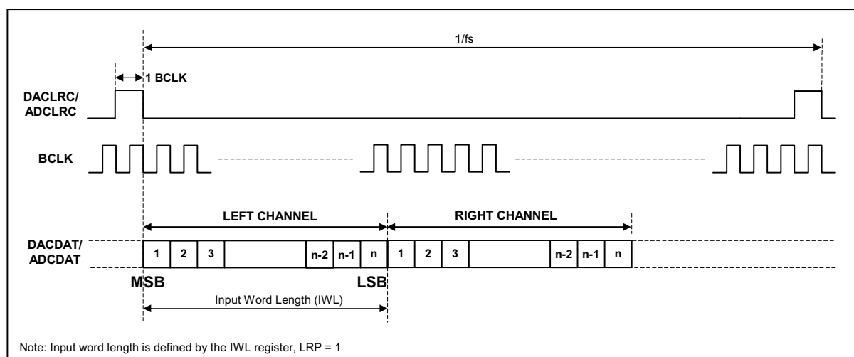
Figure 19 DSP Mode
