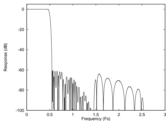
Figure 28 ADC Digital Filter Frequency Response –Type 1
