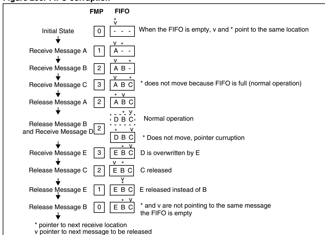
Figure 200. FIFO corruption
