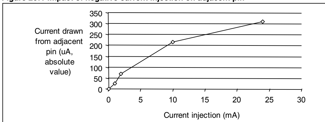
Figure 207. Impact of negative current injection on adjacent pin
