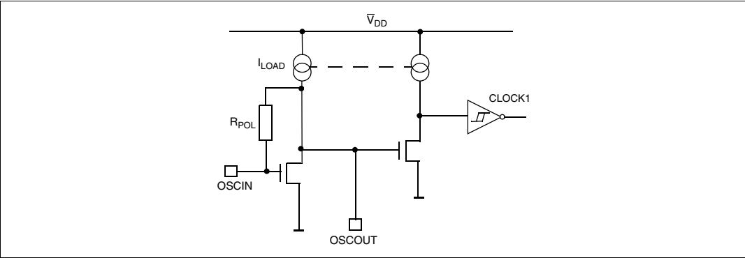
Figure 67. Internal oscillator schematic
