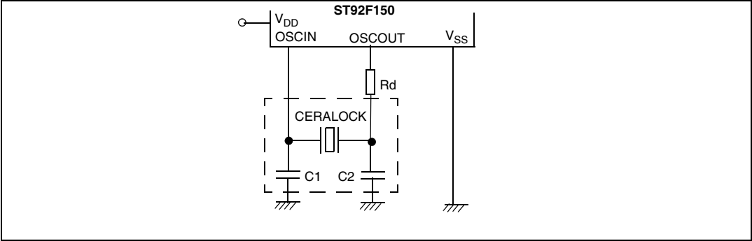
Figure 69. Test circuit
