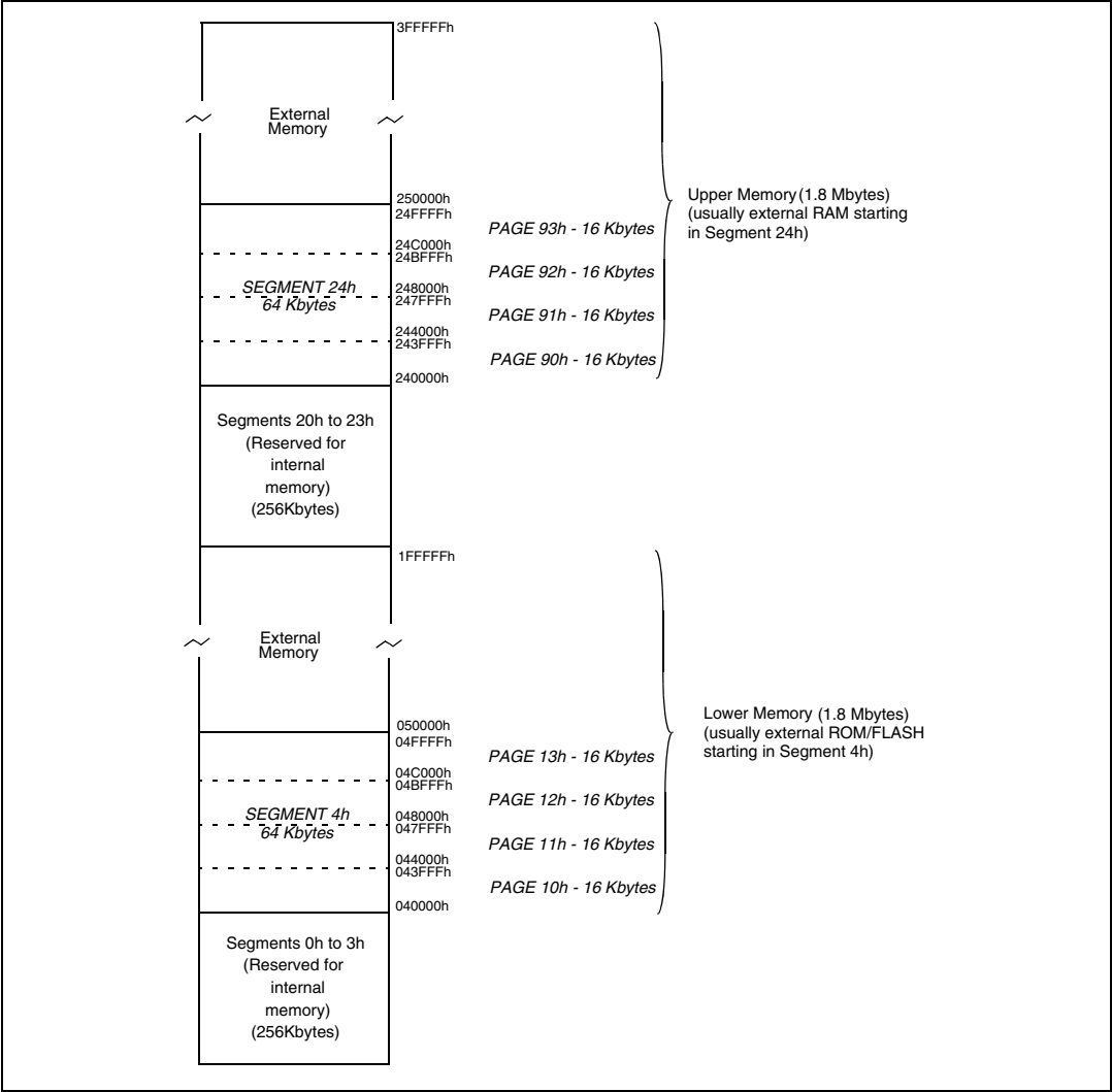
Figure 39. ST92150-Auto/250-Auto external memory map
