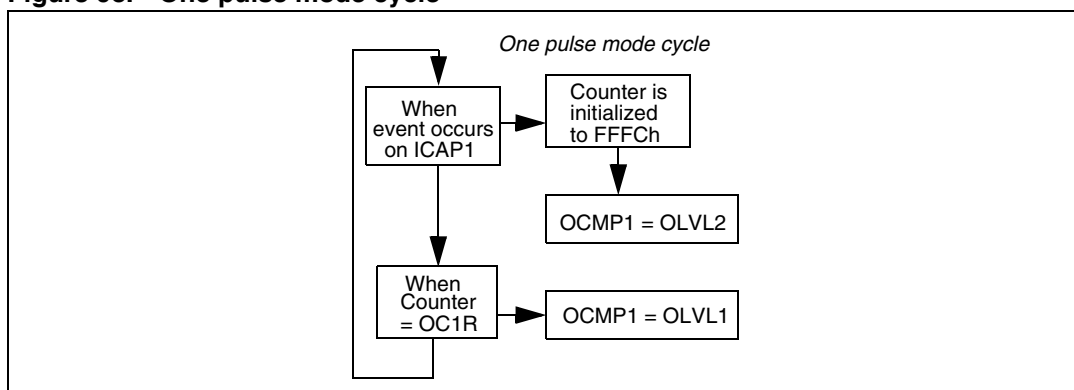
Figure 98. One pulse mode cycle
