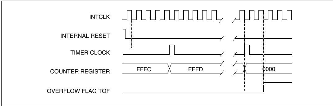
Figure 93. Counter timing diagram, INTCLK divided by 8
