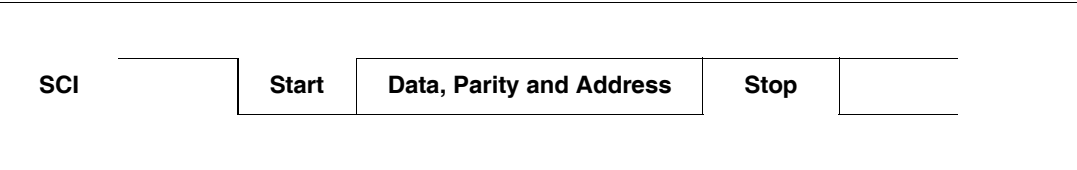
Figure 123. SCI signal
