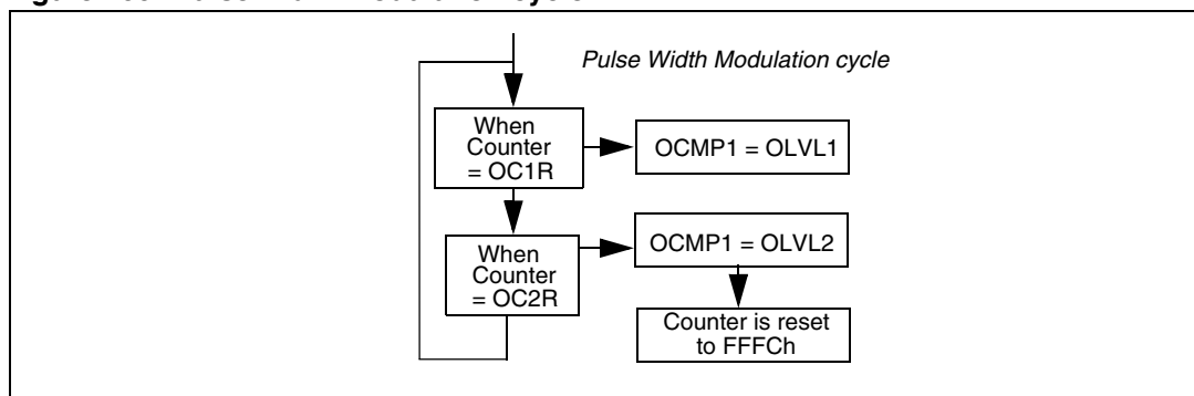
Figure 100. Pulse width modulation cycle
