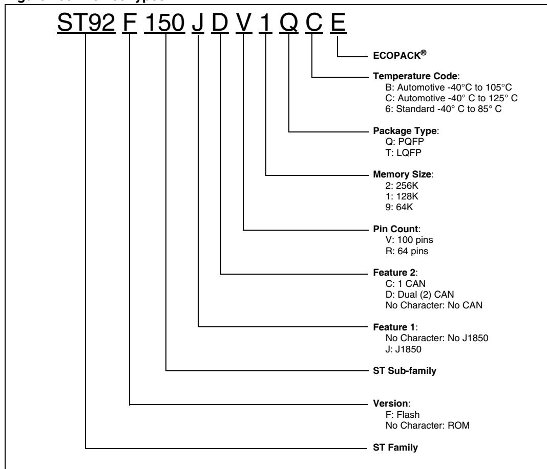
Figure 195. Device types
