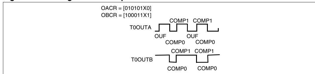
Figure 115. Configuration example 1
