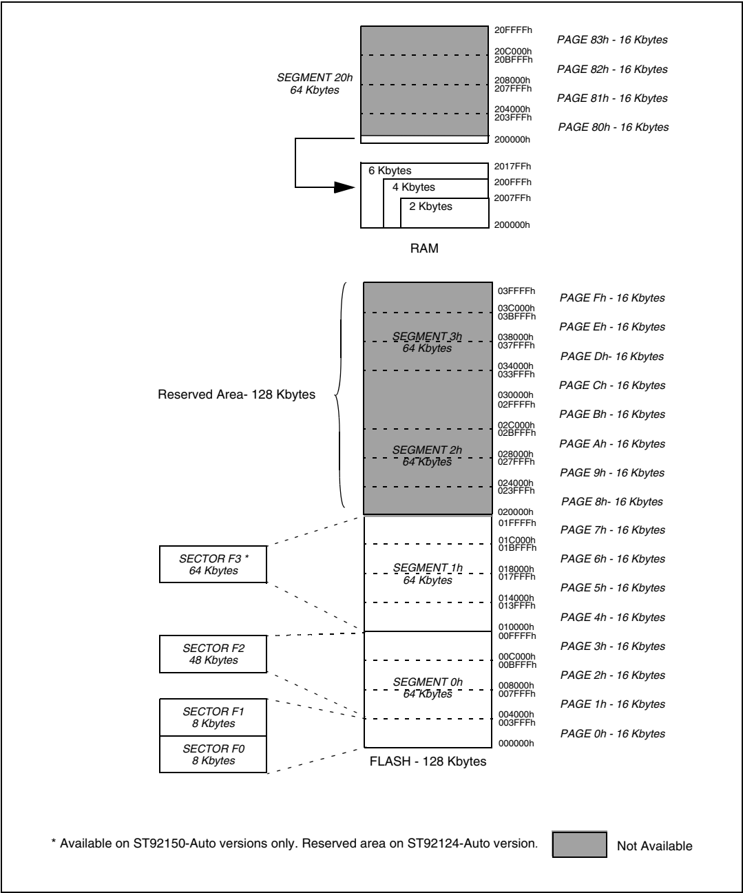
Figure 42. ST92124-Auto/150-Auto internal memory map (128K versions)
