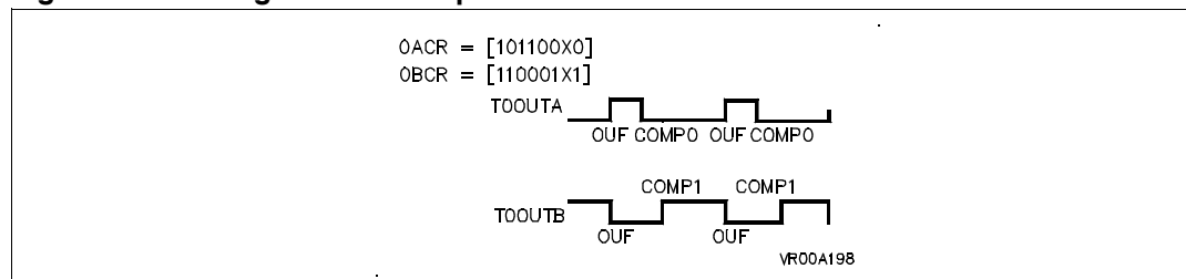
Figure 116. Configuration example 2
