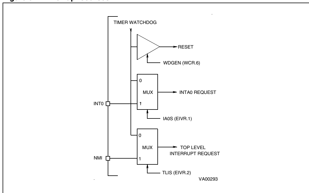
Figure 87. Interrupt sources
