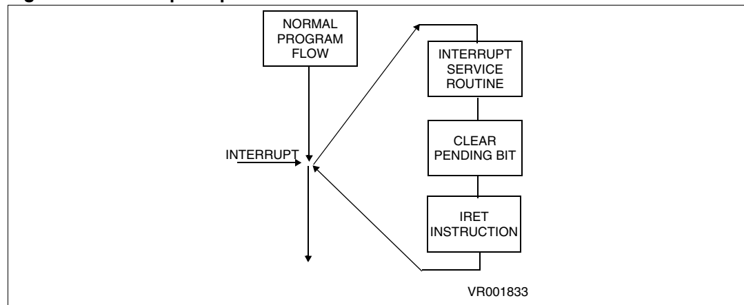
Figure 44. Interrupt response
