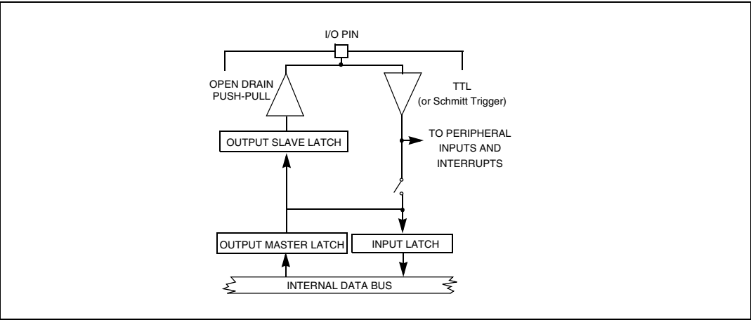
Figure 81. Output configuration
