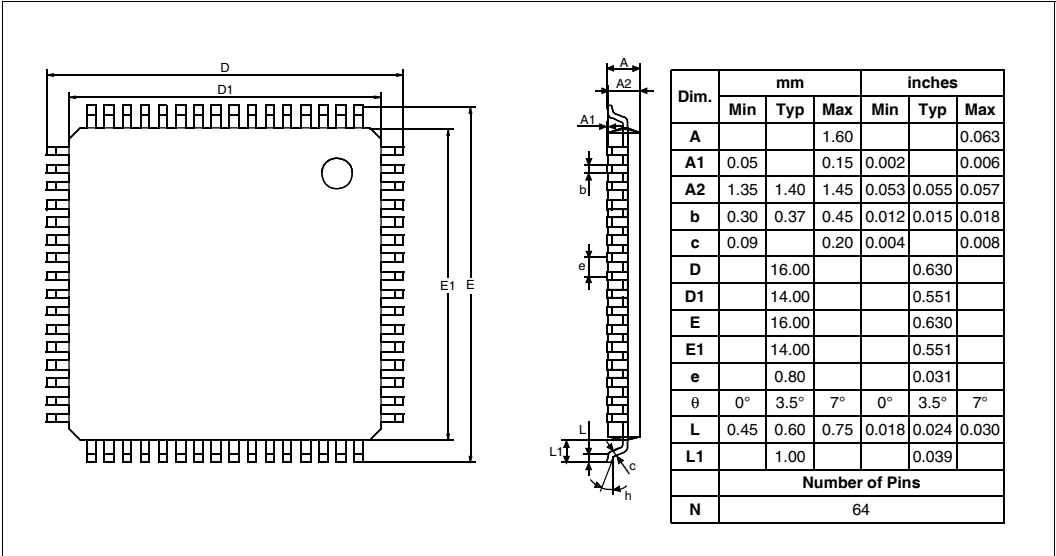
Figure 196. 64-pin low profile quad flat package
