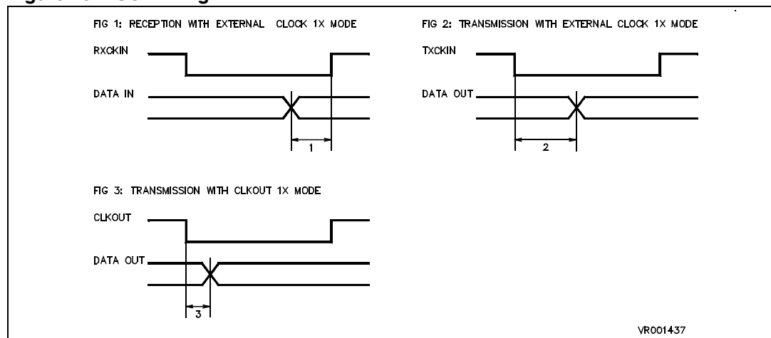
Figure 182. SCI timing
