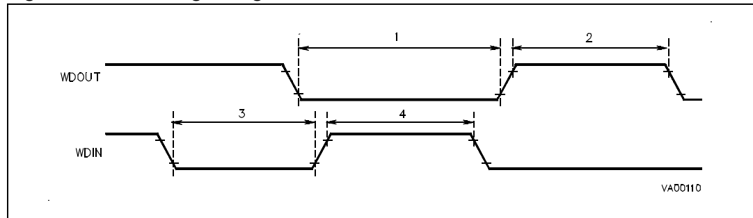
Figure 178. Watchdog timing
