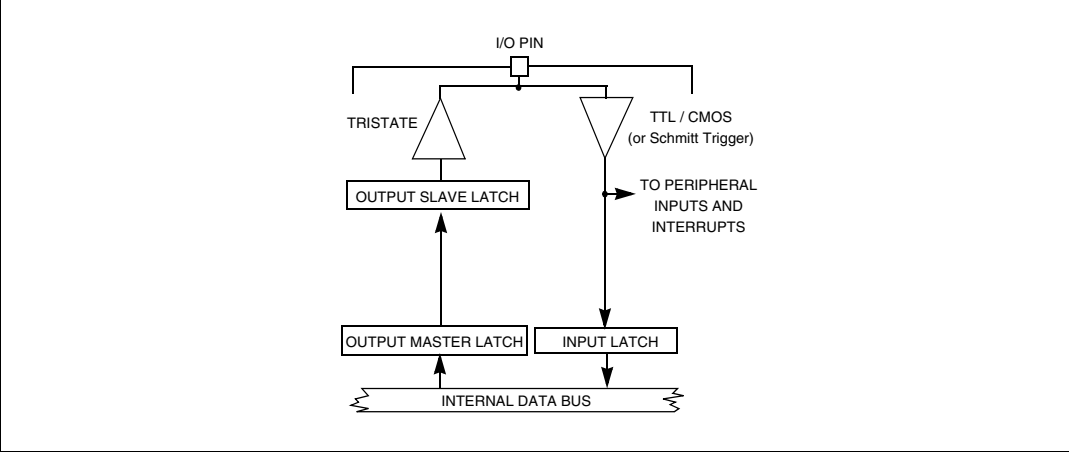
Figure 80. Input configuration
