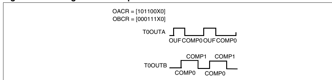
Figure 117. Configuration example 3
