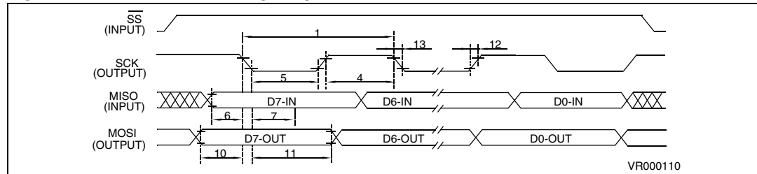
Figure 184. SPI master timing diagram CPHA=0, CPOL=1
