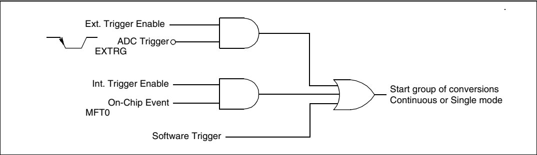
Figure 171. ADC trigger source
