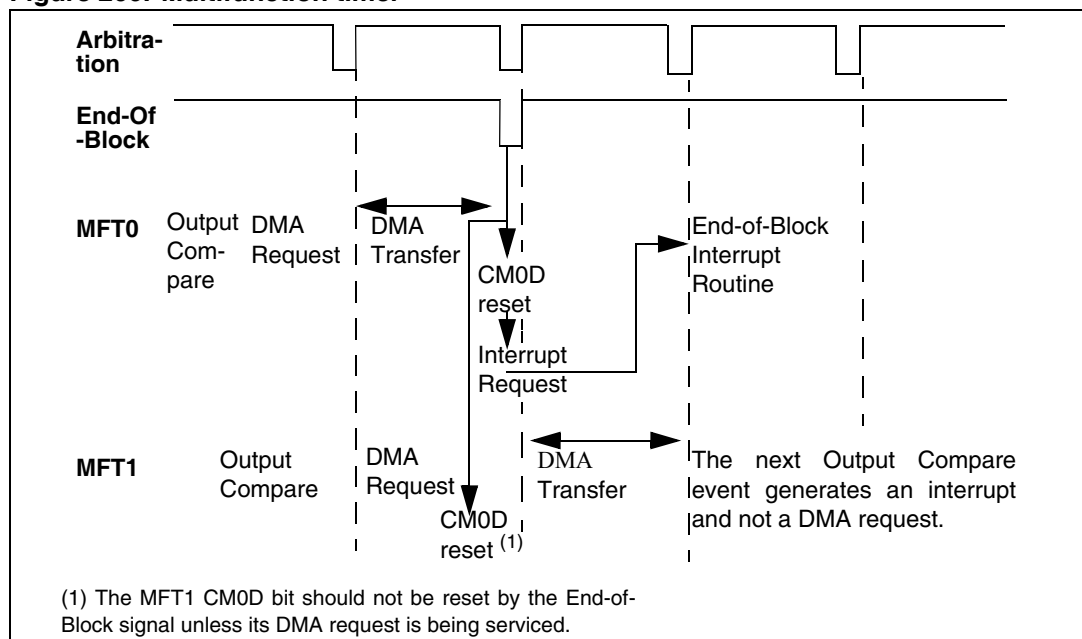
Figure 206. Multifunction timer
