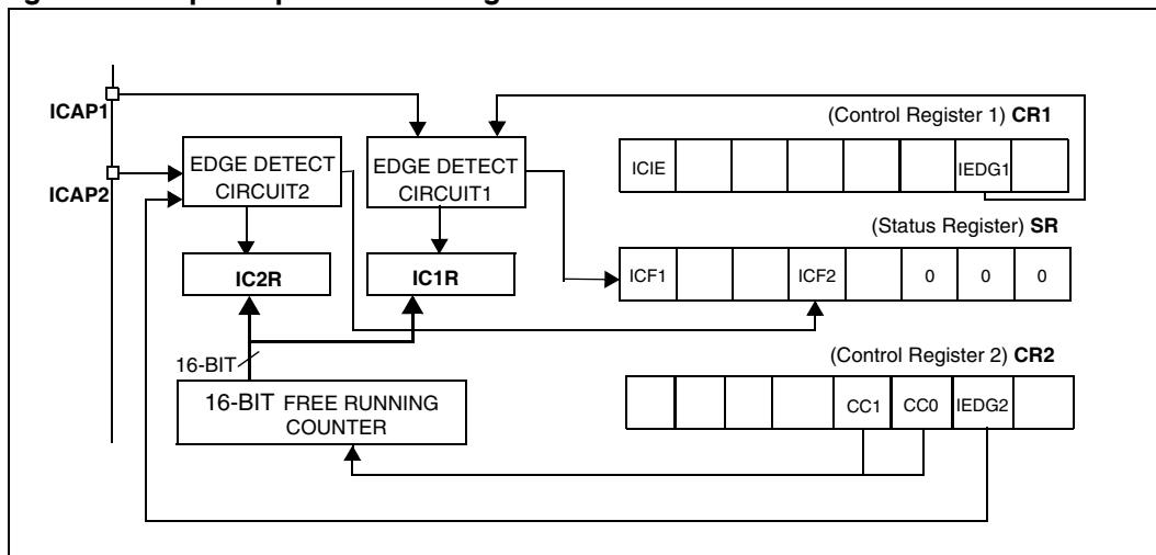
Figure 94. Input capture block diagram
