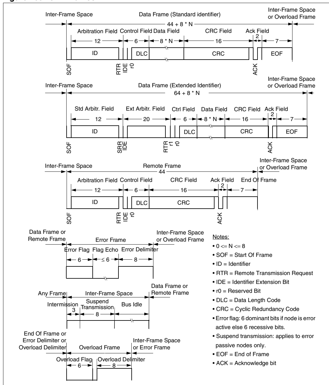
Figure 165. CAN frames
