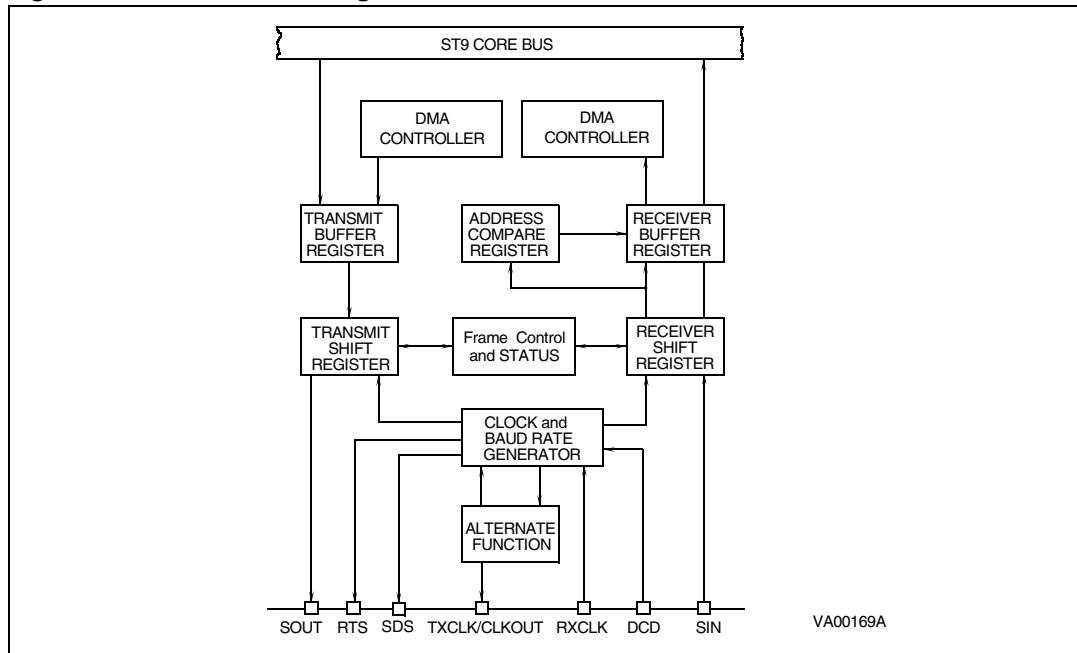
Figure 119. SCI-M block diagram
