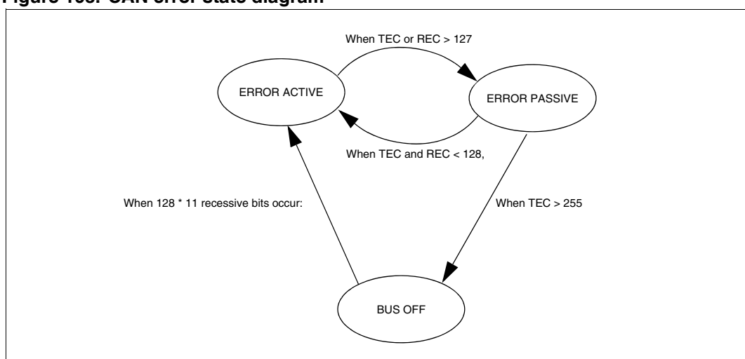
Figure 163. CAN error state diagram
