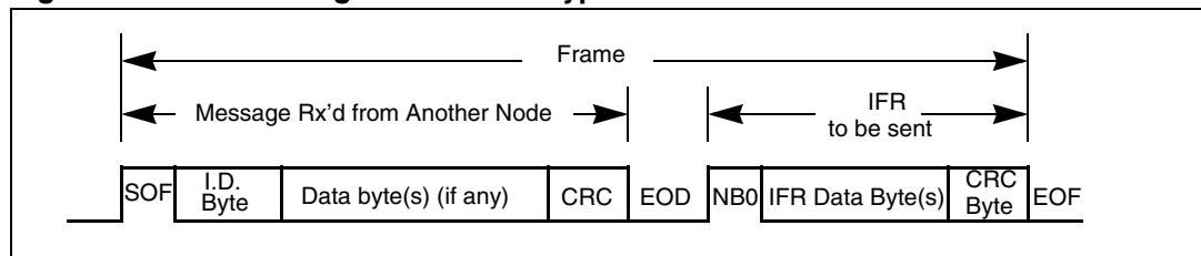
Figure 145. J1850 string transmission type 3
