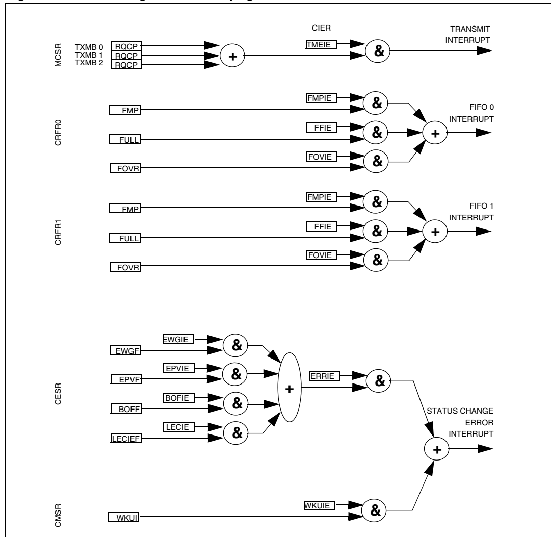
Figure 166. Event flags and interrupt generation
