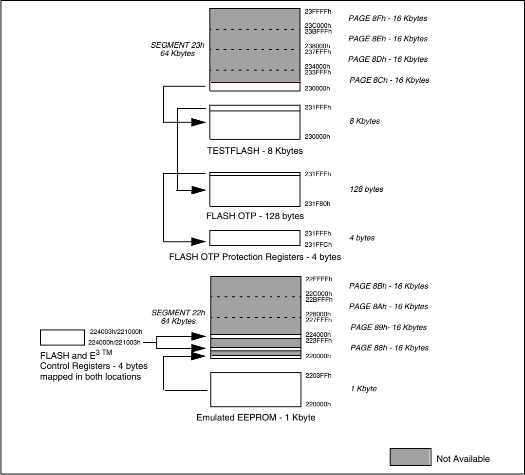
Figure 40. ST92124-Auto/150-Auto/250-Auto TESTFLASH and E 3 ™ memory map
