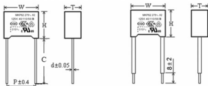
Lead Wire
