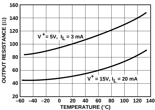
Output Resistance vs. Temperature
