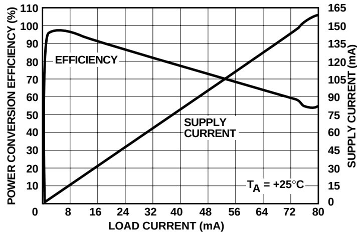
Power Conversion Efficiency vs. I_{LOAD}
