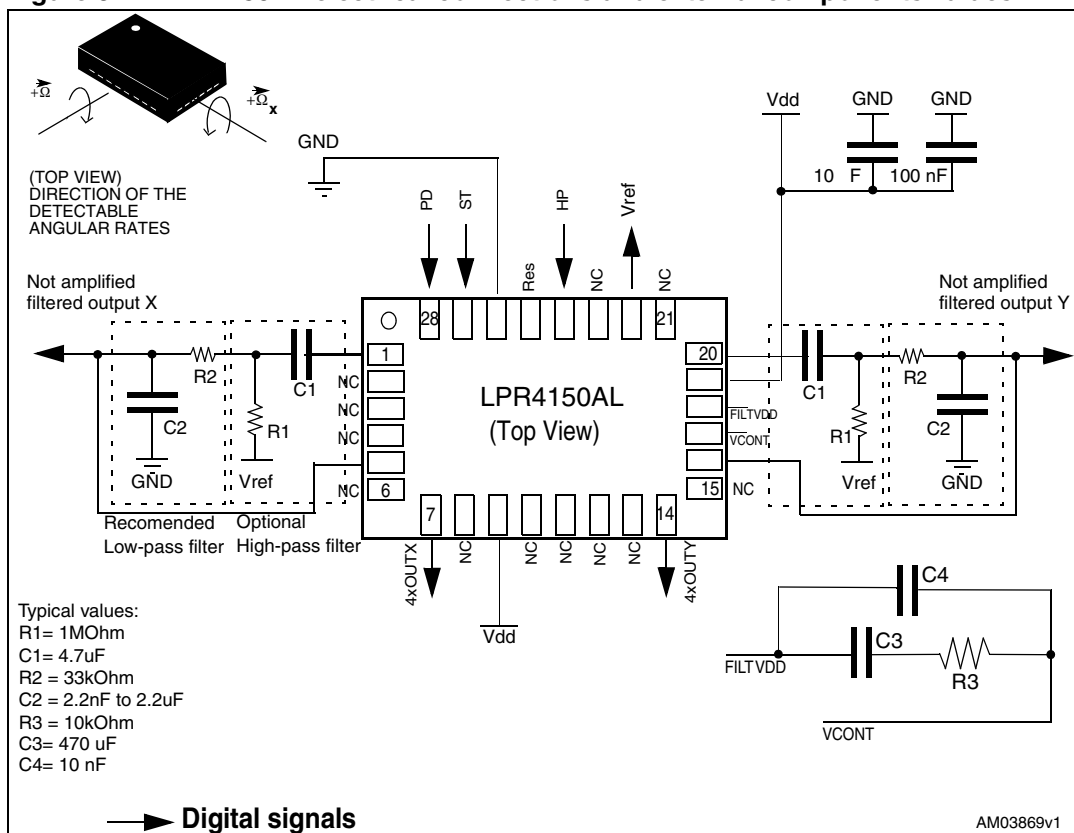
Figure 3. LPR4150AL electrical connections and external components values
