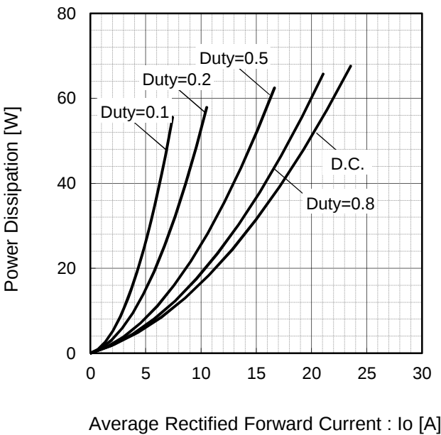
Fig.8 Io-Pf Characteristics
