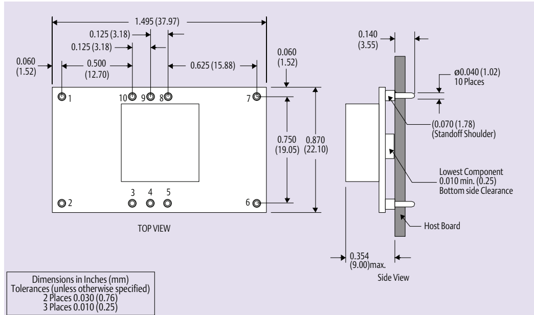
Figure 9 - Plated Through-Hole
