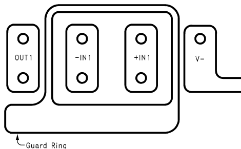
Figure 32. Example of Guard Ring in P.C. Board Layout
