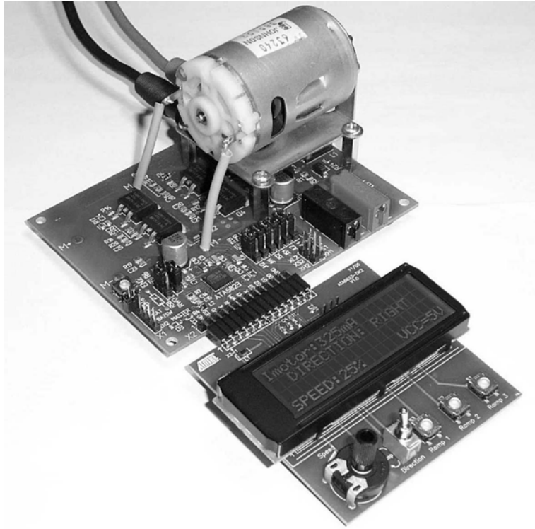
Figure 2-1. Application Board
