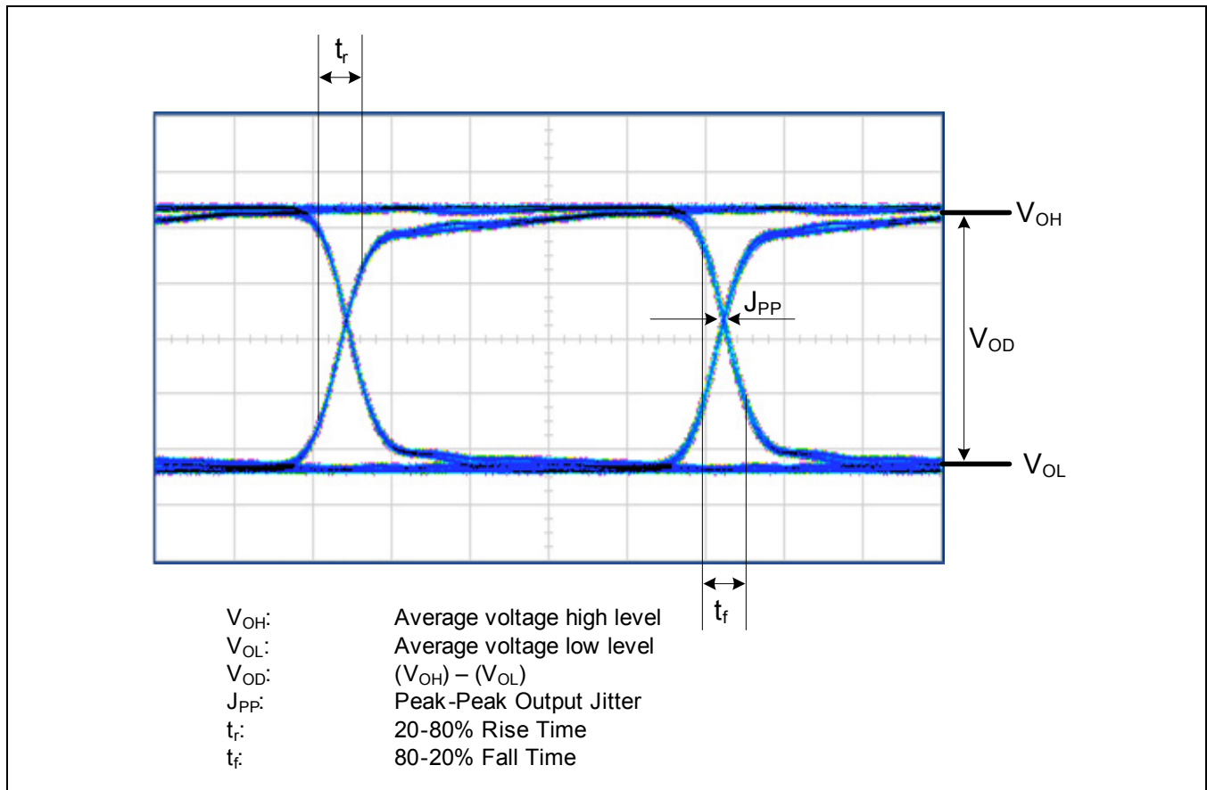
Figure 2-2. Definitions of Eye Parameters
