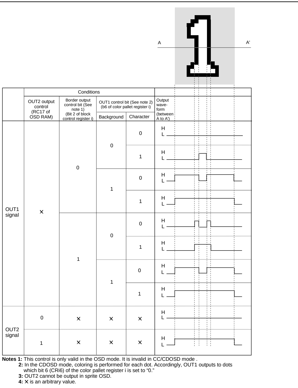
Fig. 8.11.29 Setting Value for Controlling OUT1, OUT2 and Corresponding Output Waveform
