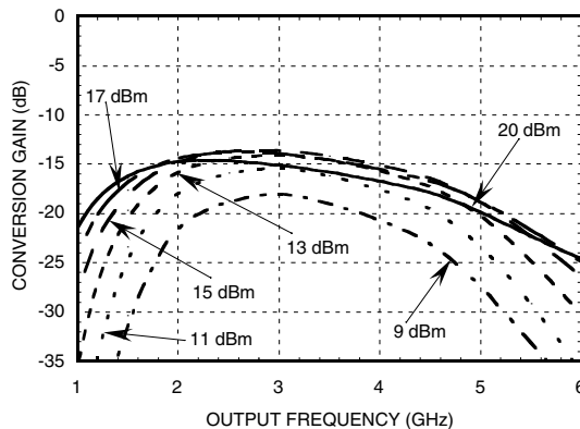
Conversion Gain @ +85°C vs. Drive Level
