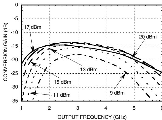
Conversion Gain @ -40°C vs. Drive Level
