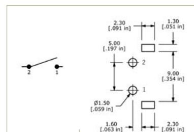
SCHEMATIC
