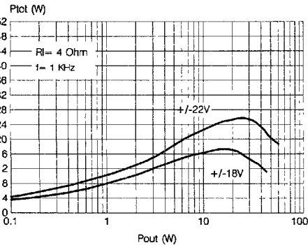
Figure 13: Power Dissipation vs. Output Power
