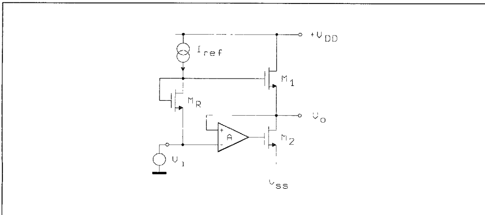
Figure 15: Principle Schematic of a DMOS unity-gain buffer.
