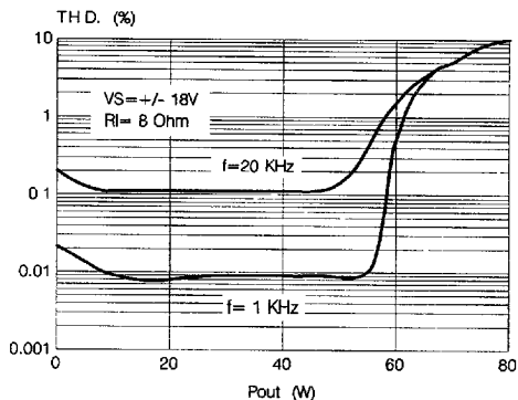
Figure 20: Distortion vs. Output Power
