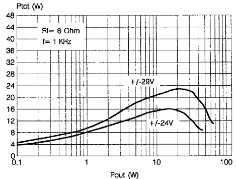
Figure 14: Power Dissipation vs. Output Power
