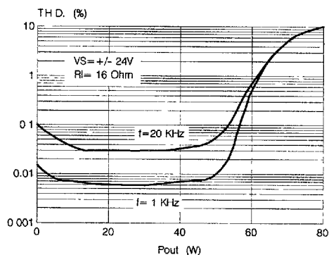
Figure 21: Distortion vs. Output Power
