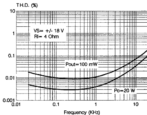
Figure 8: Distortion vs. Frequency
