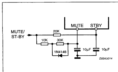
Figure 17: Single Signal ST-BY/MUTE Control Circuit
