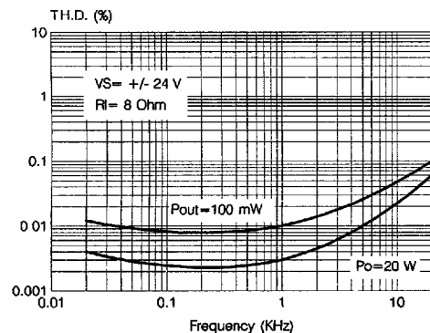
Figure 7: Distortion vs. Frequency
