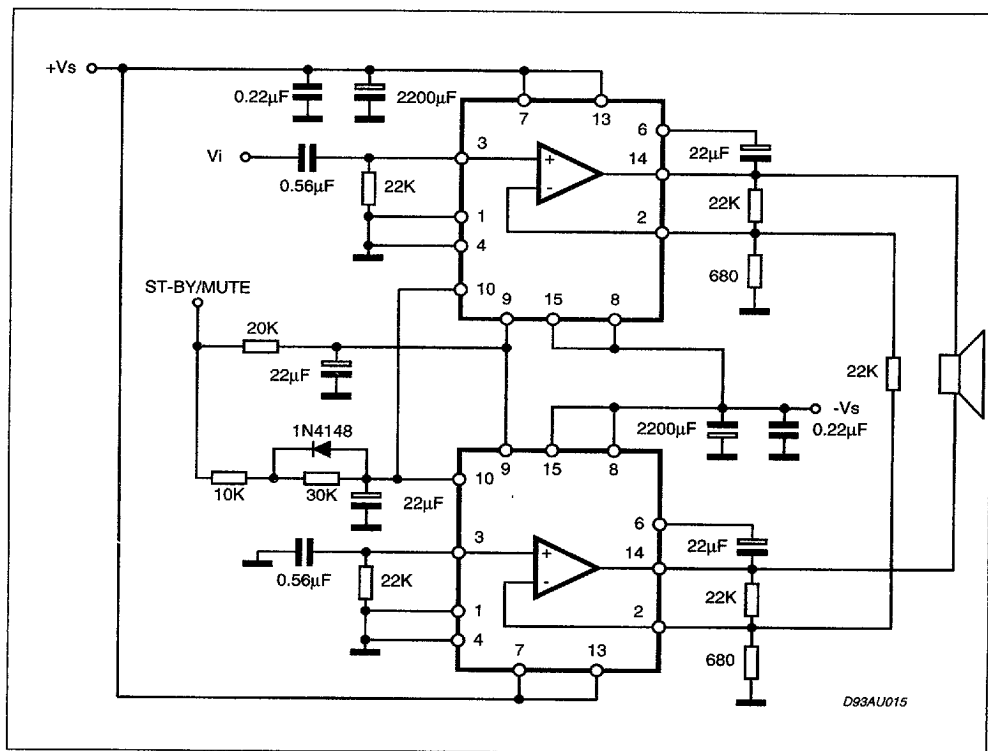
Figure 18: Bridge Application Circuit
