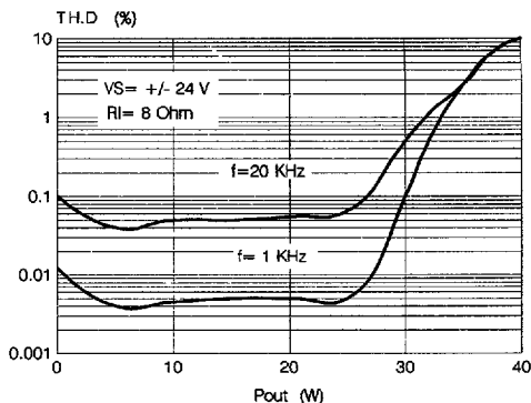
Figure 6: Distortion vs. Output Power
