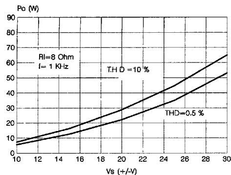
Figure 5: Output Power vs. Supply Voltage
