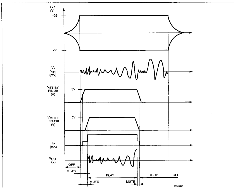
Figure 16: Turn ON/OFF Suggested Sequence
