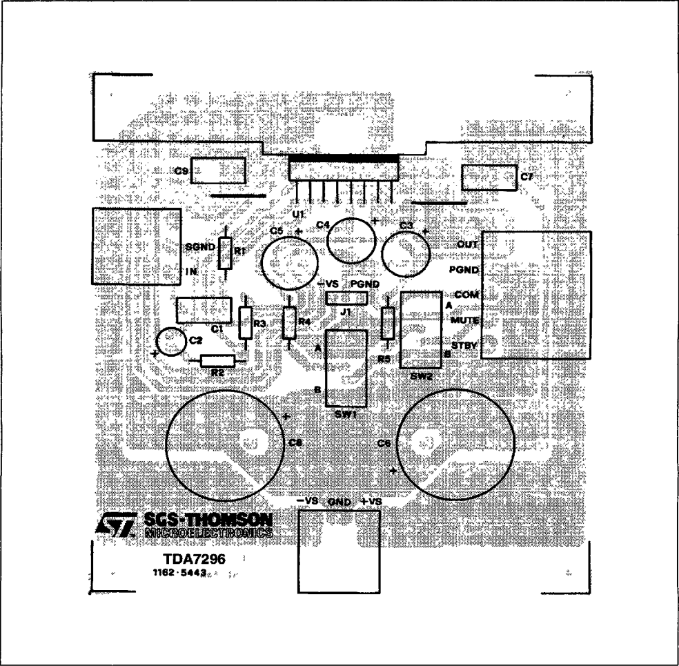
Figure 2: P.C.B. and components layout of the circuit of figure 1. (1:1 scale)
