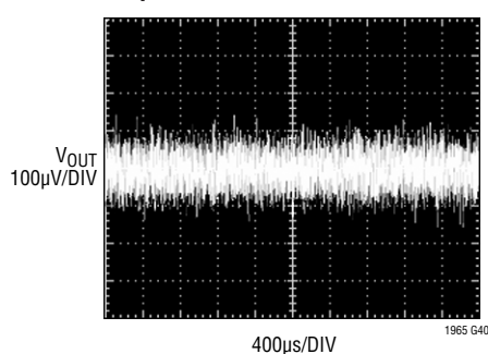
LT1965-1.8 10Hz to 100kHz Output Noise
