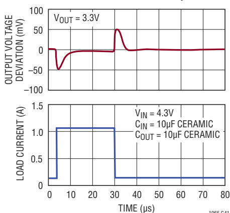
LT1965-3.3 Transient Response
