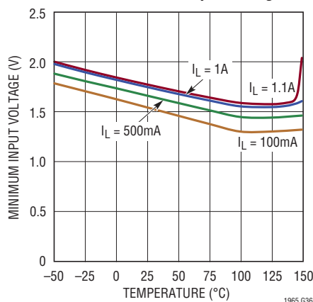
LT1965 Minimum Input Voltage
