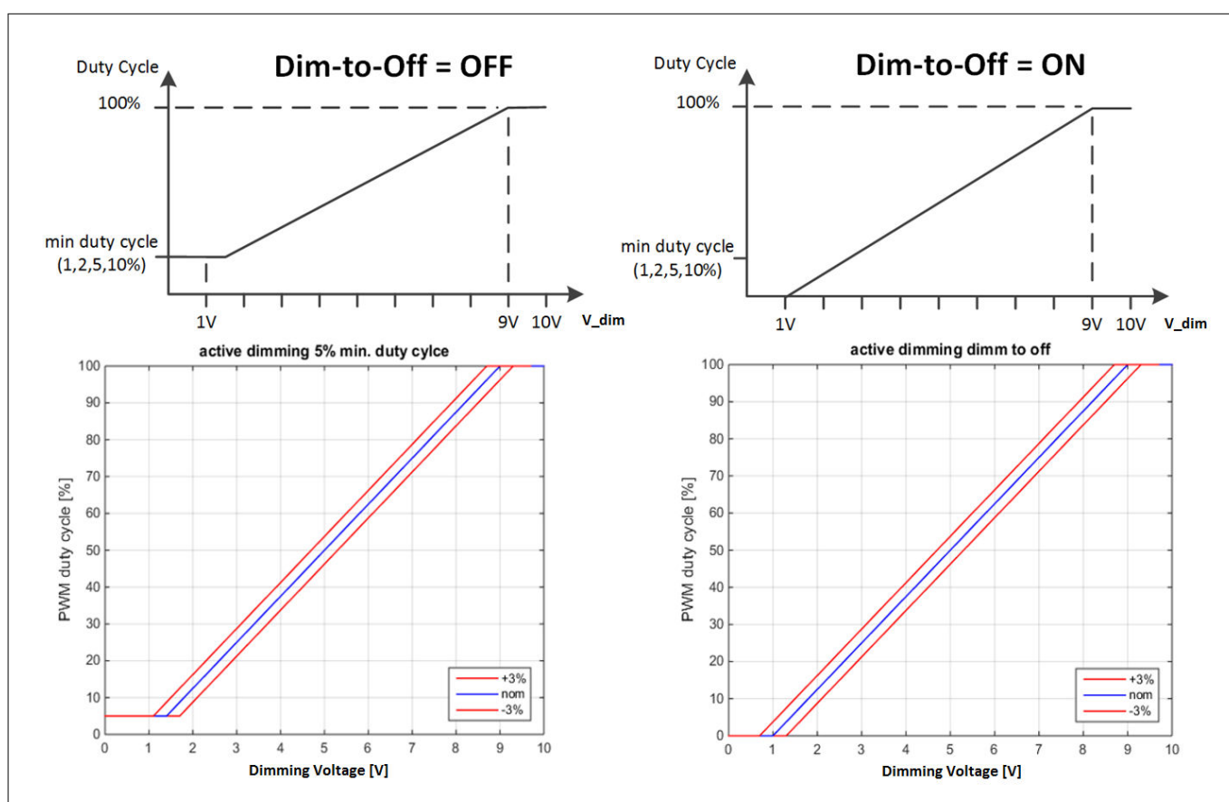
Figure 4 Dimming Characteristic
