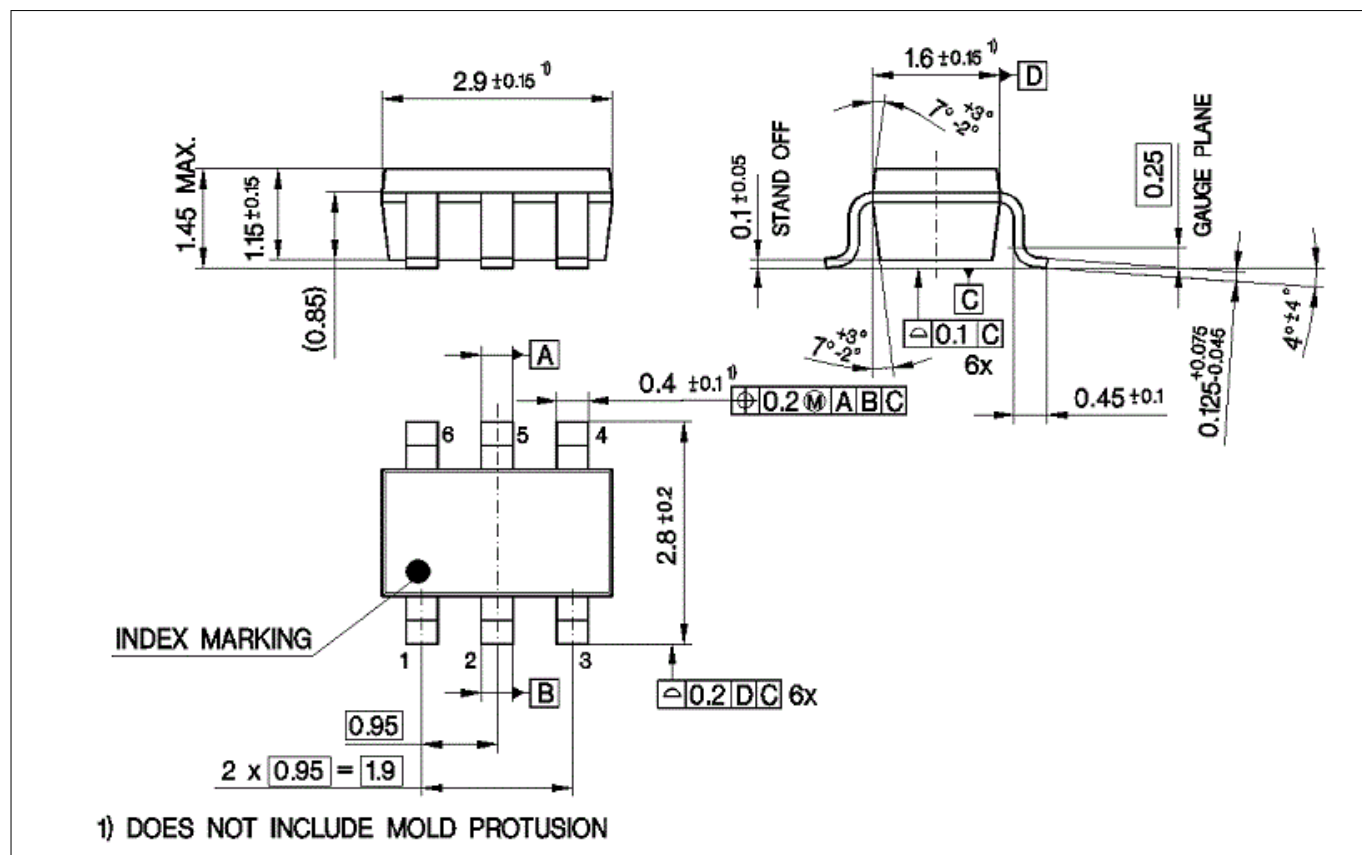
Figure 13 Package Drawings
