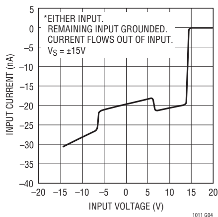
Input Characteristics*
