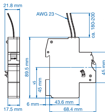
Dimensions UA120UM.
