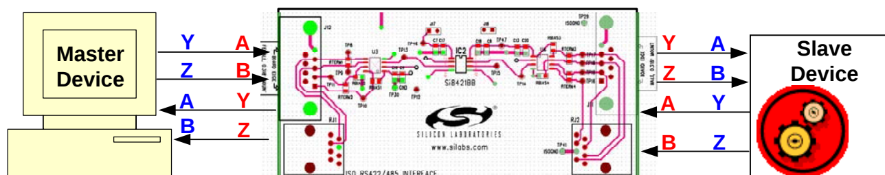
Figure 8. Simple Point-to-Point RS422/485 Connection
