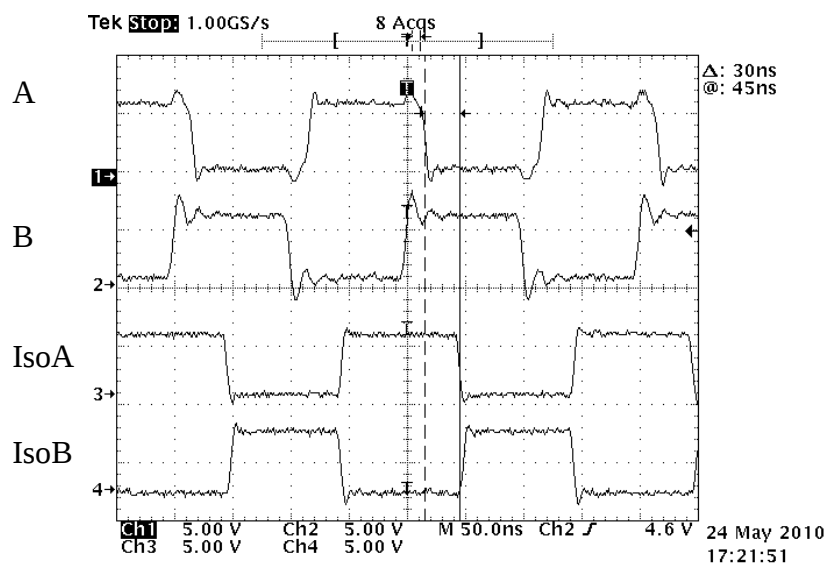
Figure 12. Isolated RS422/485 Signals (Unterminated) at 10 Mbps
