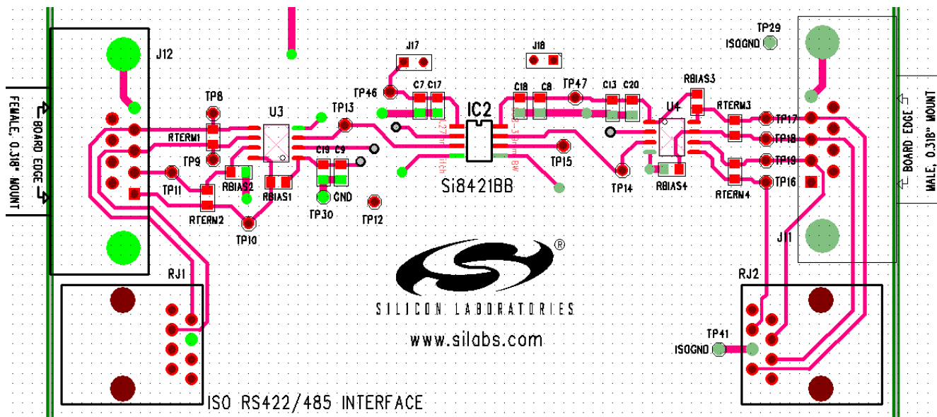
Figure 4. Isolated 4-Wire RS422/485 Interface
