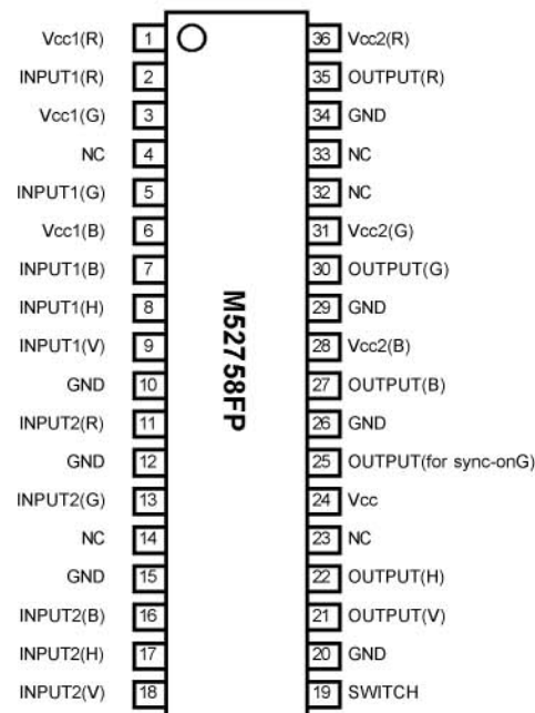
Outline 36P2R-D
