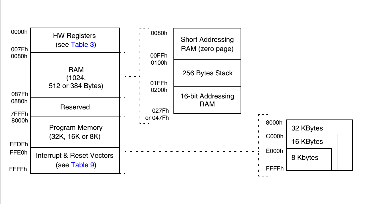
Figure 6. Memory Map
