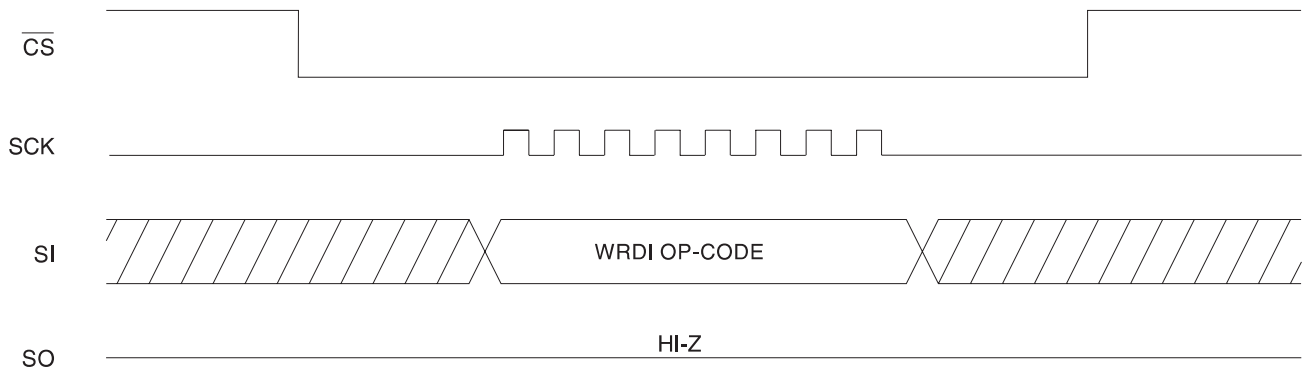
Figure 3-3. WRDI Timing
