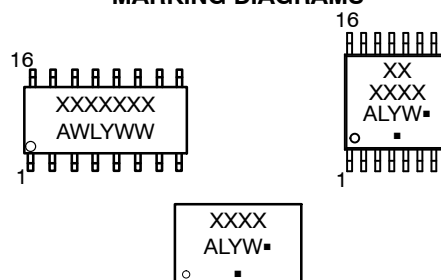
QFN16 MN SUFFIX CASE 485AW
