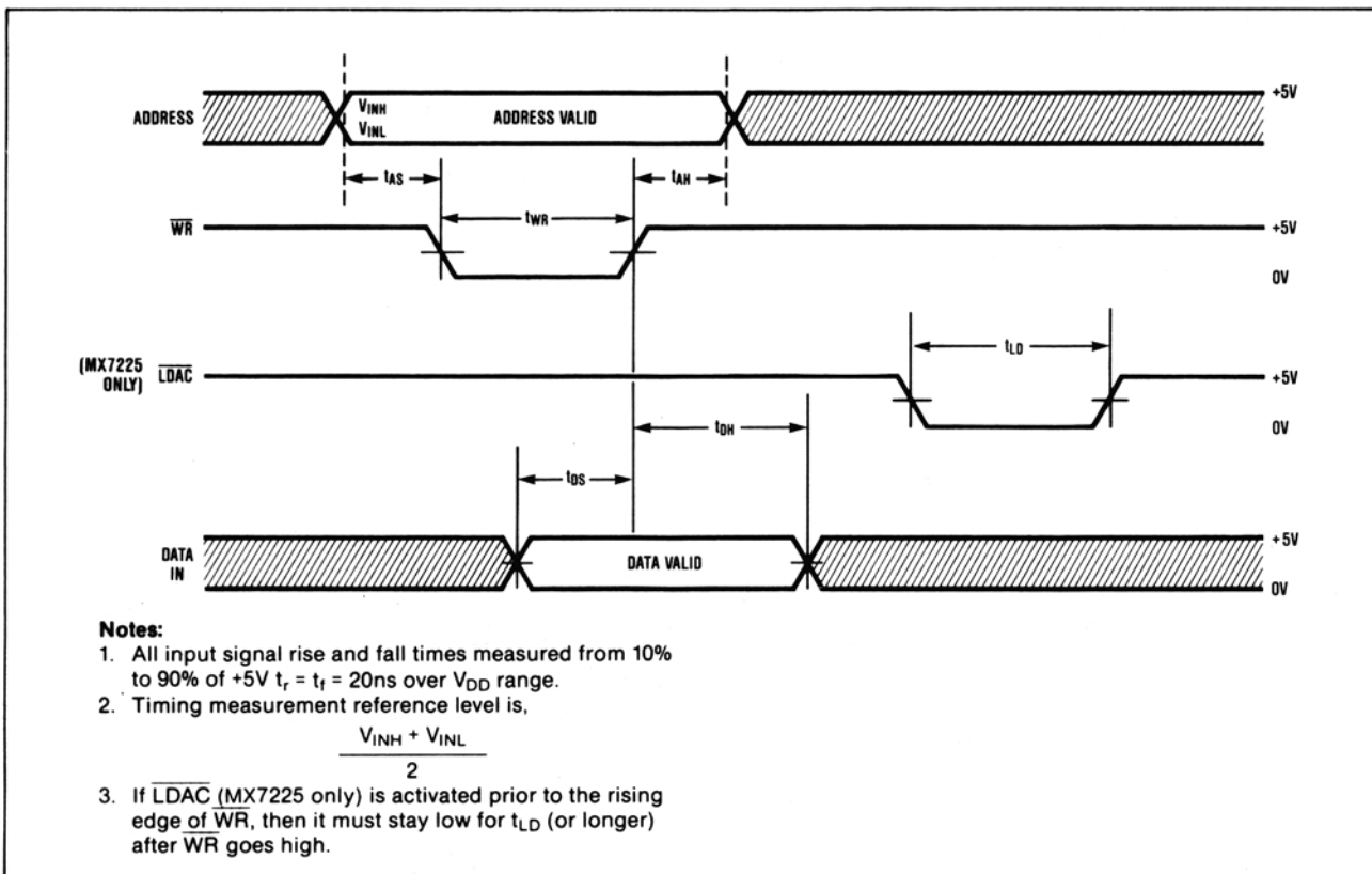
Figure 6. Write Cycle Timing Diagram
