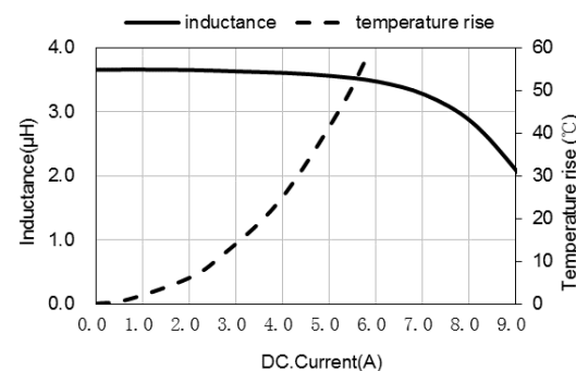
ASPIAIG-S8050-3R3
