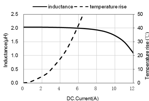
ASPIAIG-S8050-2R2
