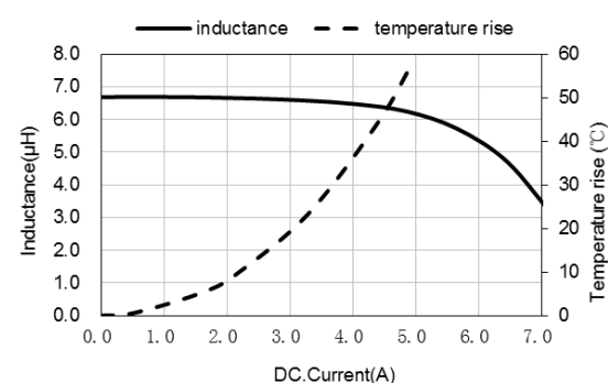
ASPIAIG-S8050-6R8
