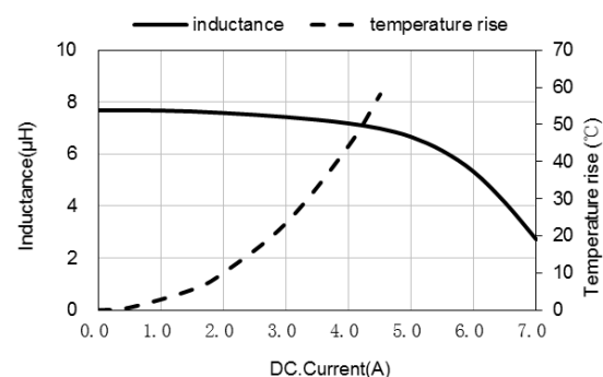
ASPIAIG-S8050-8R2
