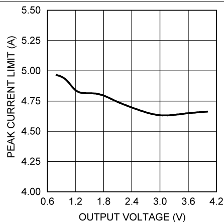
Figure 20. Peak Current Limit vs V_{OUT}
