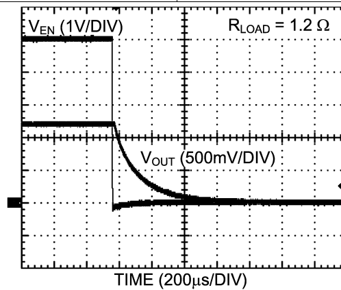
Figure 27. Power Down
