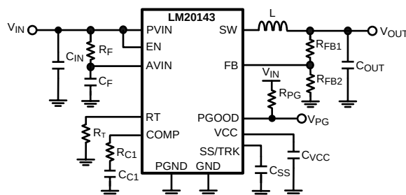
Figure 32. Typical Application Circuit
