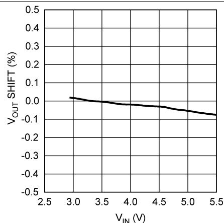
Figure 10. Line Regulation
