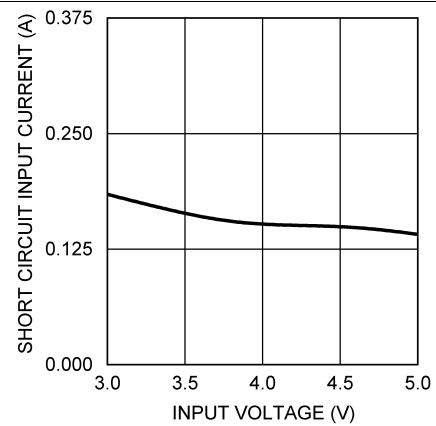
Figure 26. Short Circuit Input Current vs V_{IN}
