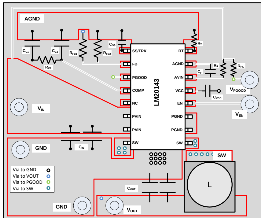
Figure 41. Example Layout
