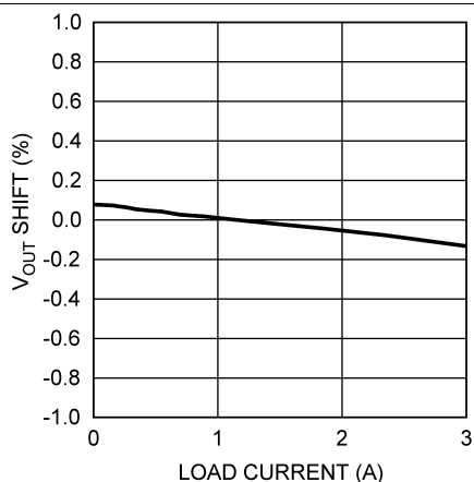
Figure 11. Load Regulation
