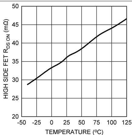
Figure 7. High-Side FET Resistance vs Temperature
