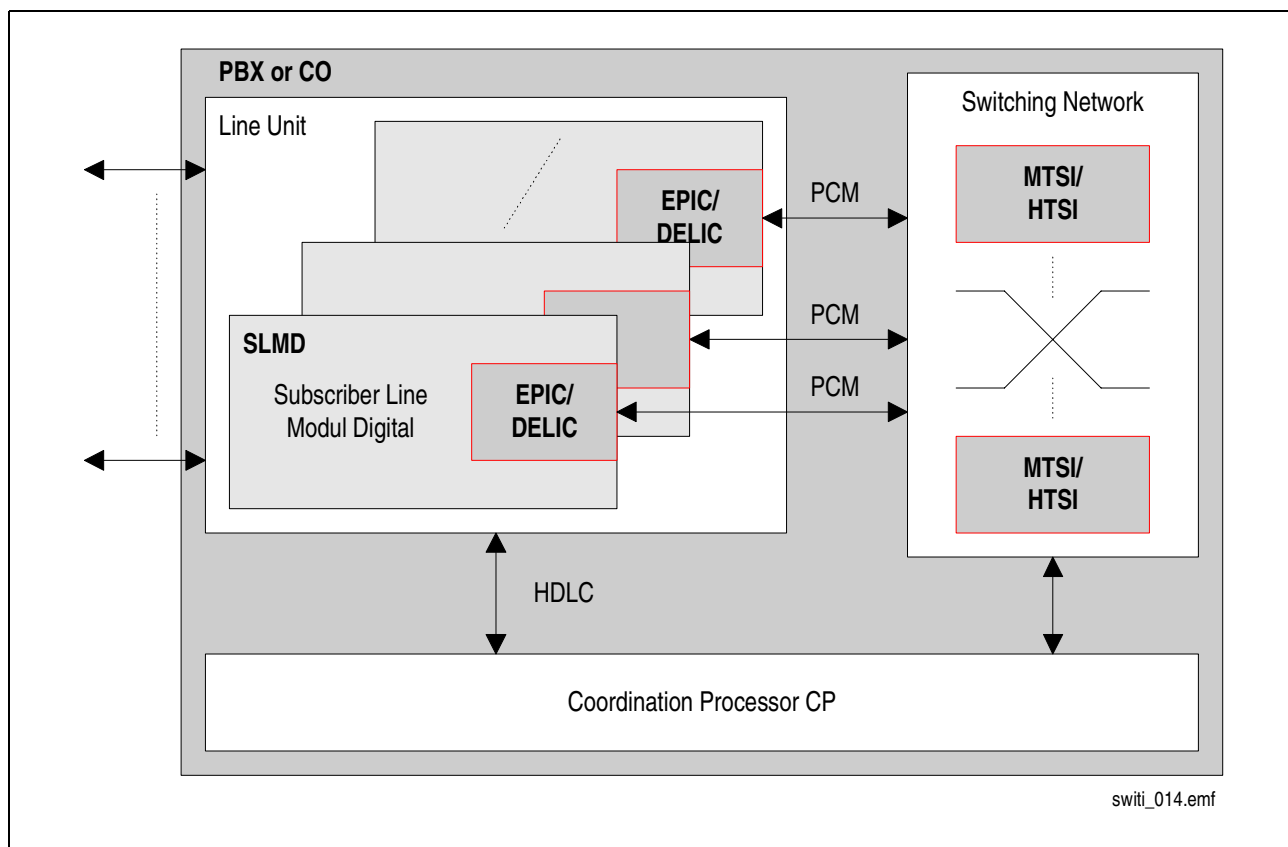
Figure 2 Standard PBX or CO Application
