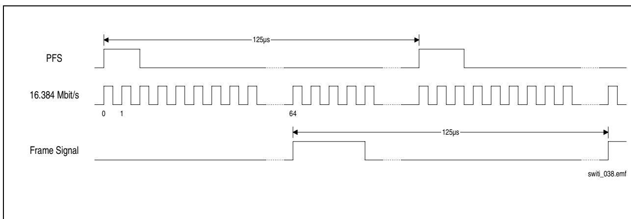
Figure 14 Frame Signal Example
