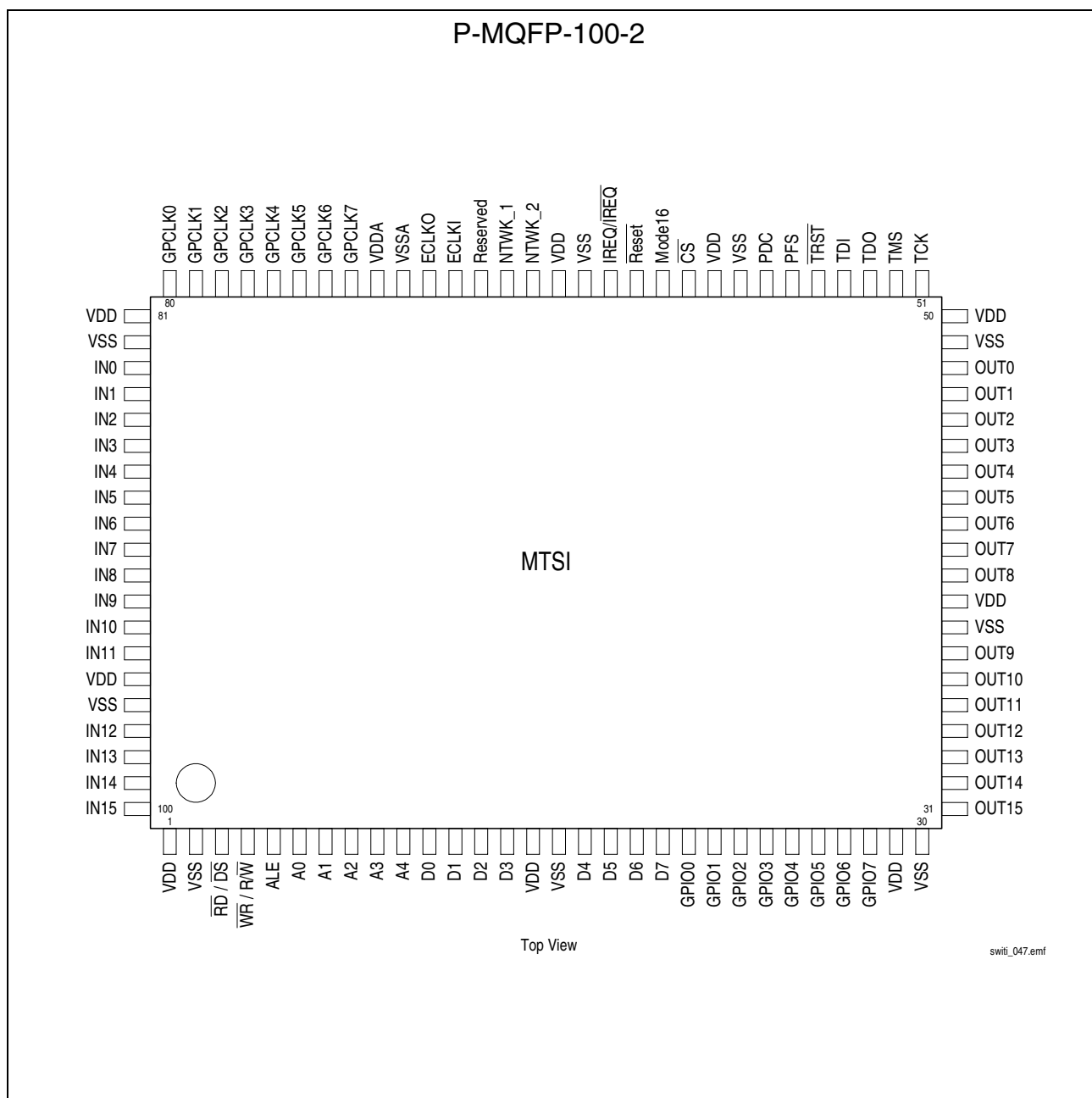
Figure 3 Pin Configuration
