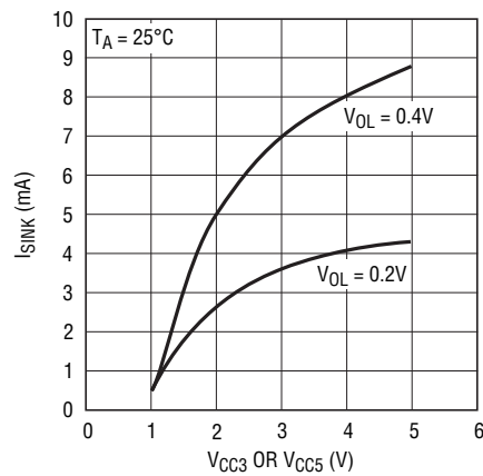
\overline{RST} , COMPX I_{SINK} vs Supply Voltage
