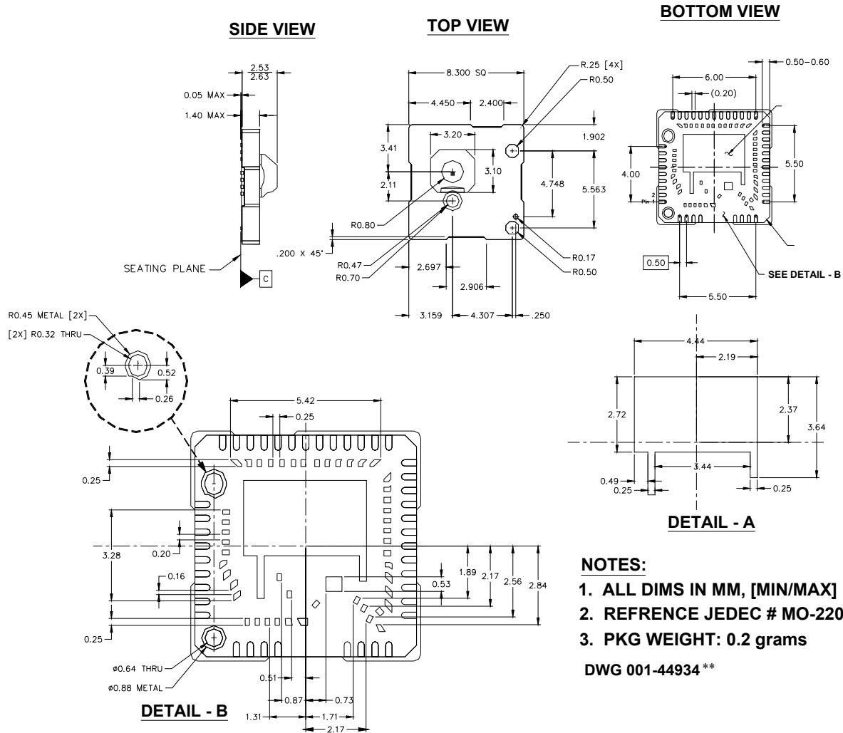
Figure 18. QFN Package
