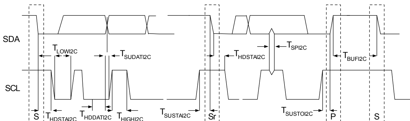
Figure 13. Timing for Fast and Standard Mode on the I 2 C Bus
