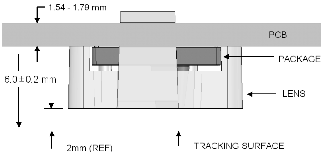
Figure 17. PCB Height and Thickness
