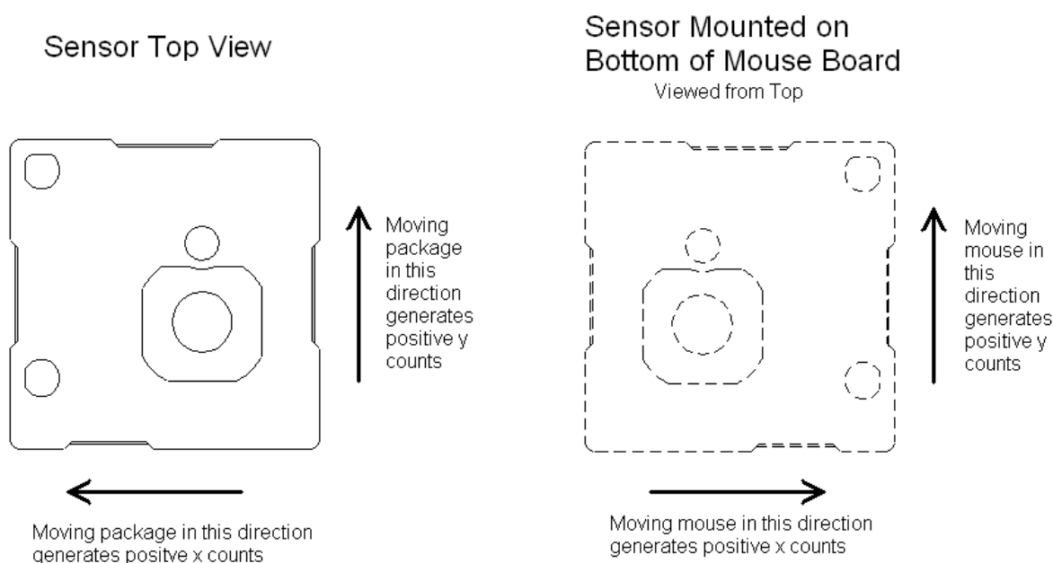
Figure 16. Sensor Orientation
