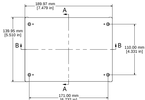
ASSEMBLY - TOP
