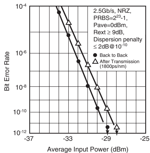
Fig. 7 Transmission Characteristics
