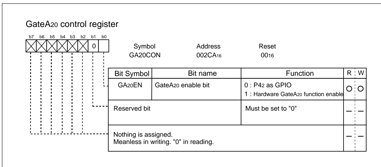
Fig.GF-9 GateA20 control register
