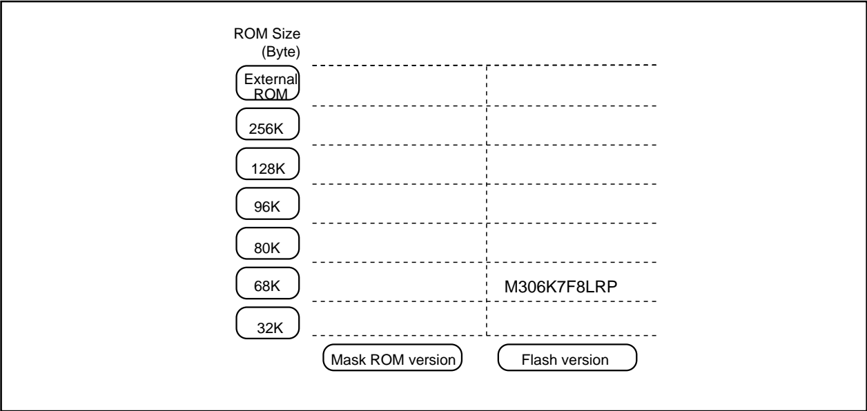
Fig.AA-3 ROM expansion
